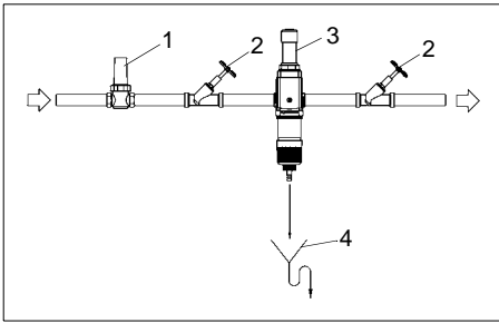
Fig. 3: Installation
