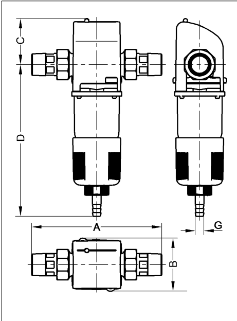
Fig. 6: Installation dimensions JEF-B \frac{3}{4} " - 1\frac{1}{4} "
